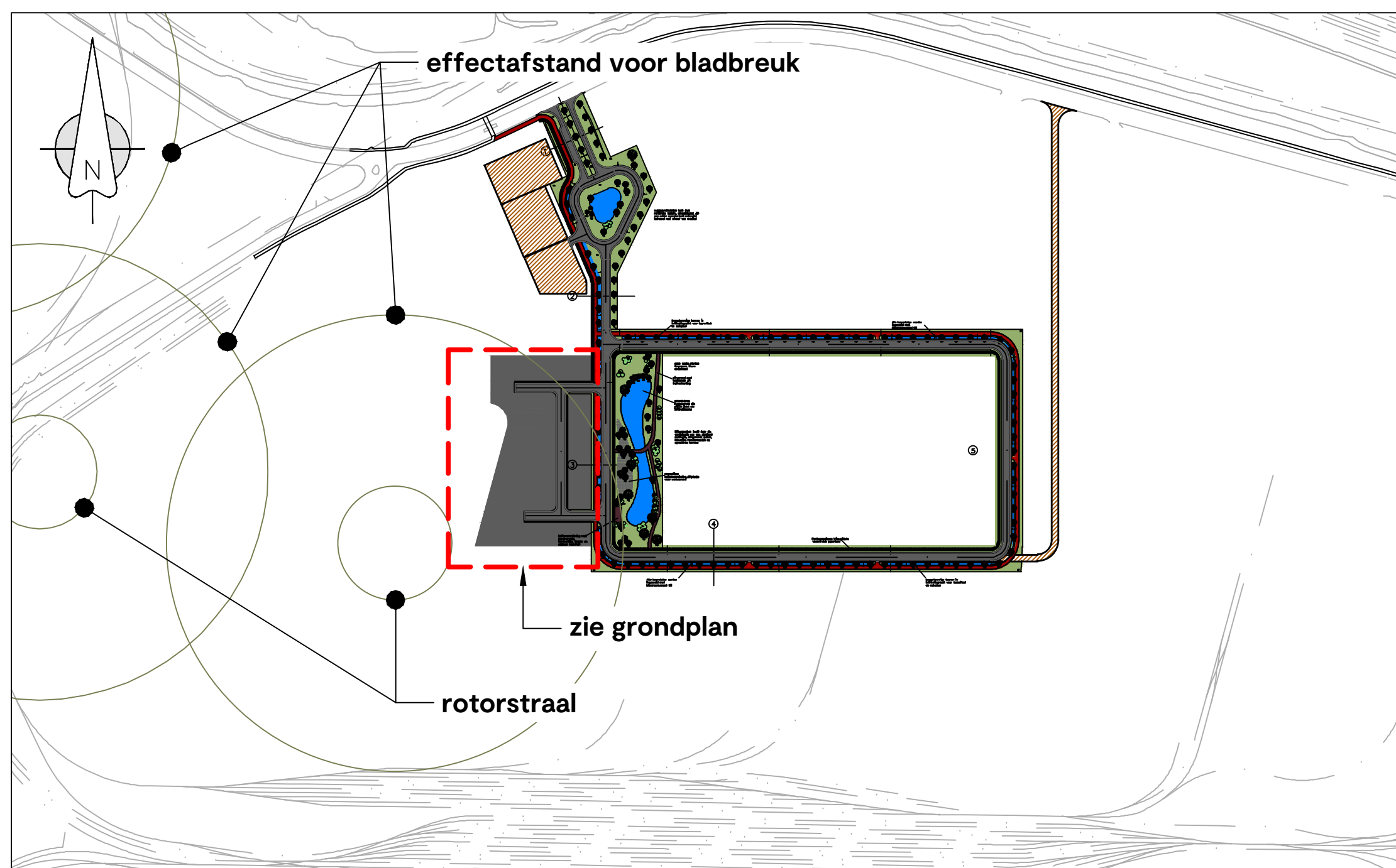
Inplantingsplan Schaal 1:5000
